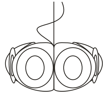
OVAL LAMPSHADE 210 MM /// 440 MM POLYPROPYLENE, POLYCARBONATE
